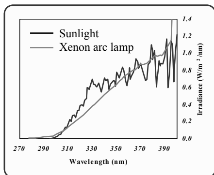
Figure 3. Irradiance output from xenon arc lamp
