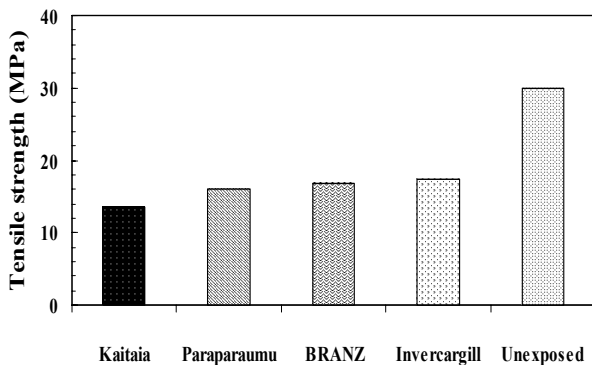
Figure 4. Tensile strengths of exposed polypropylene
