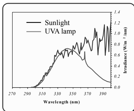
Figure 2. Irradiance output of UVA fluorescent tubes
