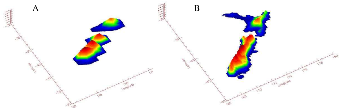
Figure 1: Representation of NZ topography by (A) Global Climate Model at resolution of 140km and (B) Regional Climate Model at resolution of 30km. Colours show the land surface elevation used in the model.
