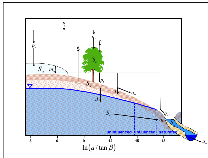
Figure 12: Main state variables and fluxes in TopNet: State variables are canopy storage ( S_c ), snowpack storage ( S_s ), soil, or root zone, storage ( S_r ), aquifer storage ( S_a ), and overland flow storage ( S_o ). Fluxes are precipitation rate ( p ), throughfall ( p_t ), canopy evaporation ( e_c ), snow melt ( m_s ), soil evaporation ( e_s ), infiltration ( i ), drainage ( d ), aquifer discharge ( q_b ), infiltration-excess runoff ( q_{ix} ), saturation-excess runoff ( q_{sx} ), basin outflow ( q_o ). The wetness index \ln(a/\tan \beta) , where a is upstream area and \beta is slope, divides the catchment into saturated and unsaturated zones.
