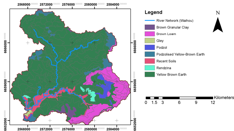
Figure 5a: Soil type in Waihou Catchment
