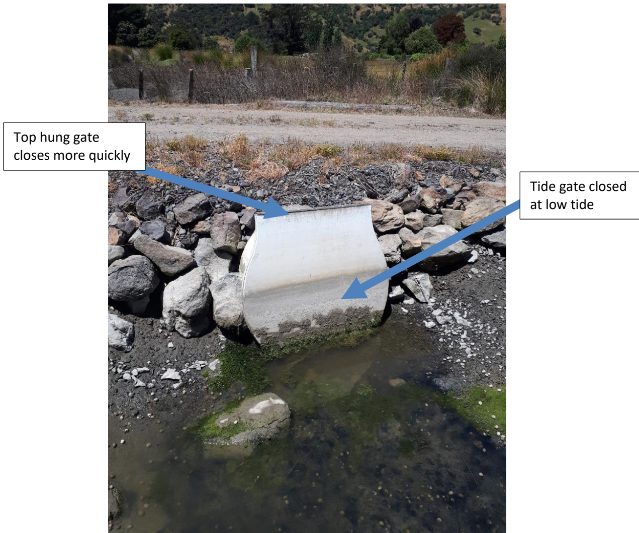
Figure B-14: Example of a culvert with a flap gate. Fish passage will be impeded by the flap gate being closed, even at low tide. Photo credit: Sam Ammon.
