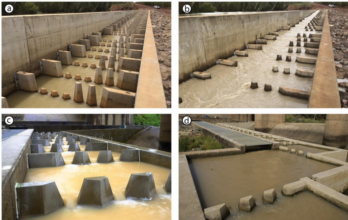
Figure 7-21: Examples of cone fishways. Panel a) and b) shows a high/low cone bypass (at Glenore weir fishway) at high and low flows. Panel c) shows a low cone bypass at the Fitzroy River Australia and d) is a tailwater stabilisation pool which improves hydraulics. Source: Stuart and Marsden (2021).
