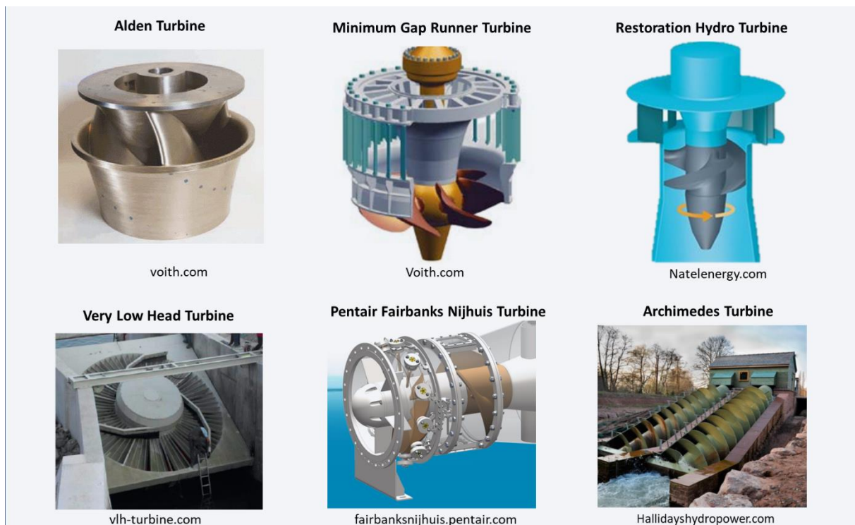
Figure 7-28: Examples of Fish friendly turbines currently used and in development internationally.
