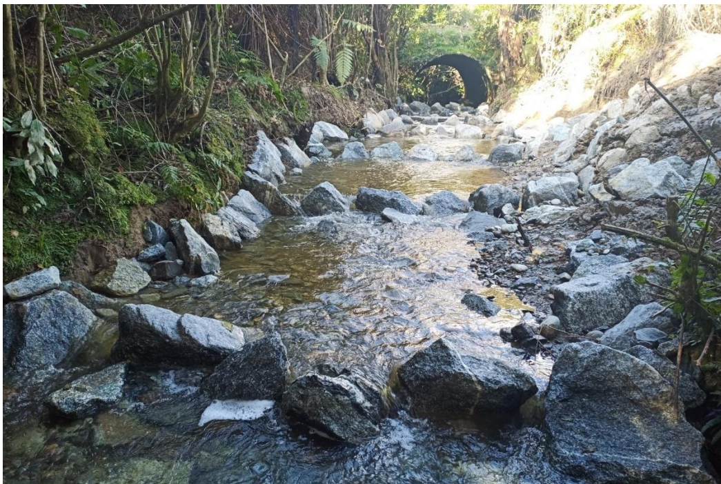
Figure 5-9: Example of a full-width rock ramp fishway in Mill Creek, West Coast. Photo credit: Koen Beets.
